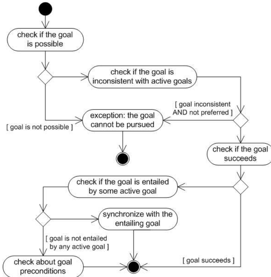
Figure 4 - The deliberation process.
