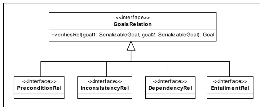
Figure 8 - Class diagram of the relations among goals in PRACTIONIST.
