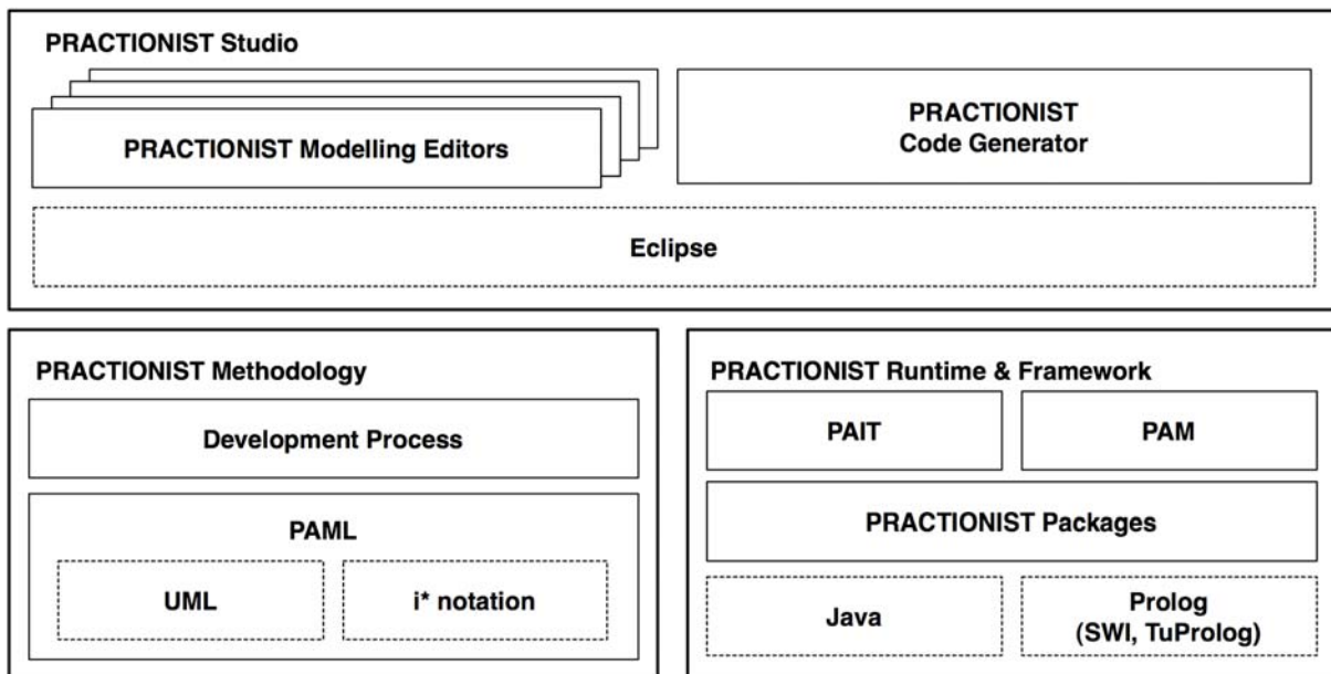
Figure 1 – The PRACTIONIST suite.
