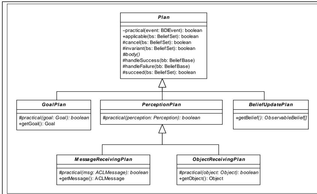
Figure 9 - Hierarchy of plans in PRACTIONIST.
