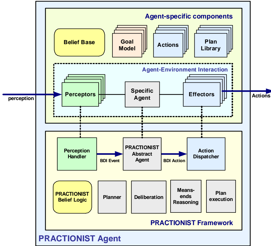
Figure 3 - Structure of a PRACTIONIST agent.
