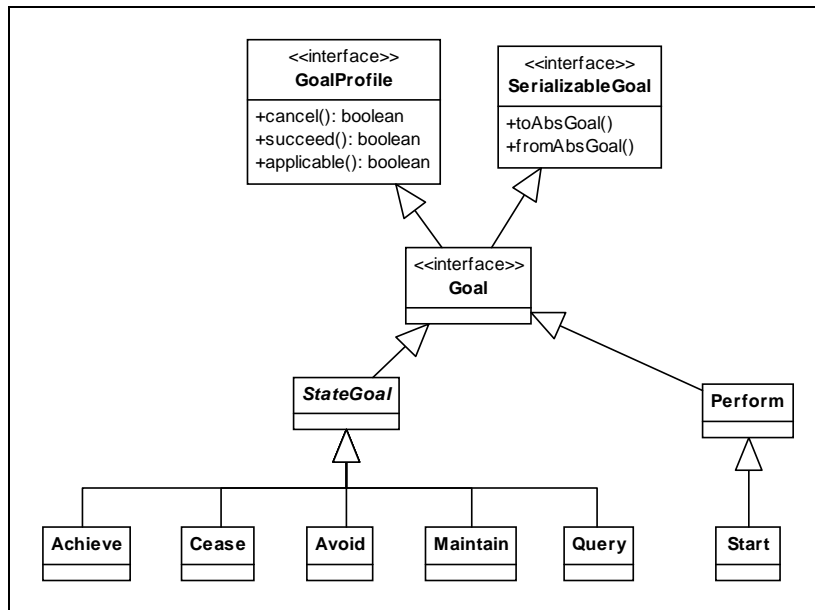
Figure 7 - Goal hierarchy in PRACTIONIST.
