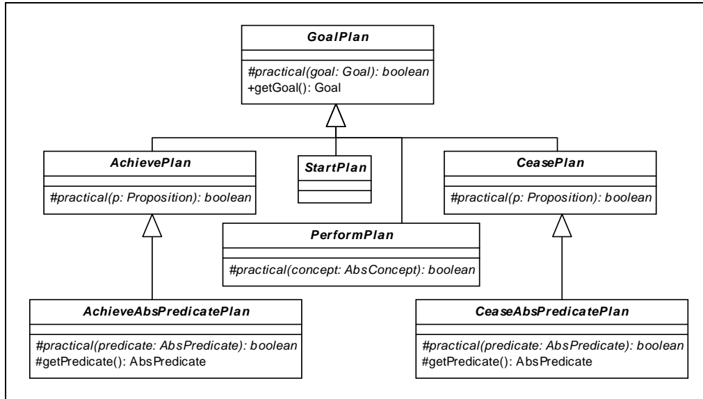
Figure 10 - Hierarchy of GoalPlan in PRACTIONIST.
