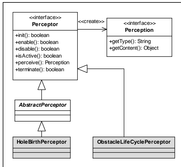
Figure 6 - Example of definition of a perceptor.
